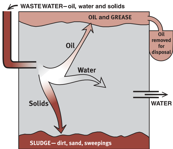
Simplified diagram of OWS operation
